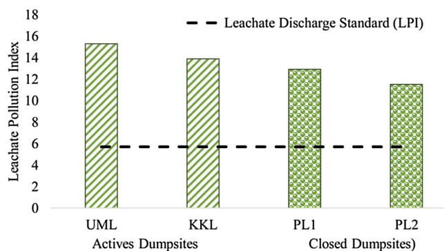
Fig. 2. Variations in leachate pollution index.
